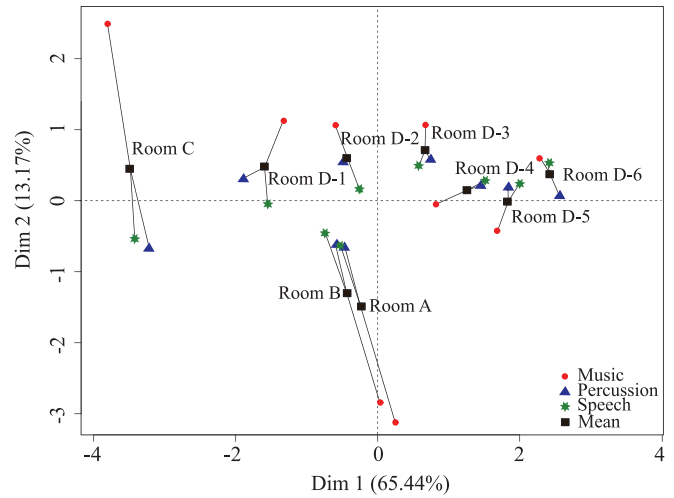
FIG. 8. Factor map showing the sensory profile of the experimental conditions. The profile is a result of three separate analyses, one for each program type. The mean is then calculated based on equally weighted contributions via the HMFA analysis, and the individual components are visualized in a common factorial space as partial points.
