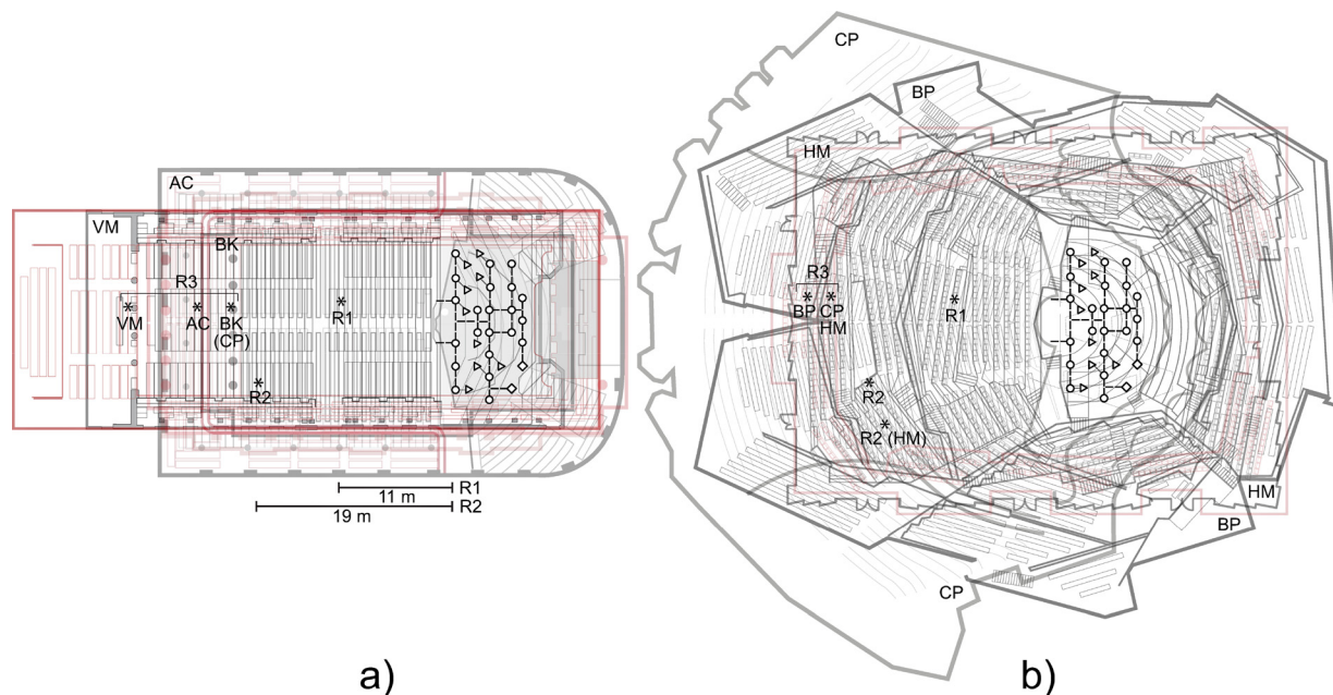
FIG. 4. (Color online) Overlaid floor plans of the (a) rectangular and (b) non-rectangular concert halls included in the listening experiment. Hall-dependent receiver positions R3 on the balcony front row are denoted with the hall abbreviations in parentheses (see Table I). Parts drawn in different shade indicate balconies above the main audience area.
