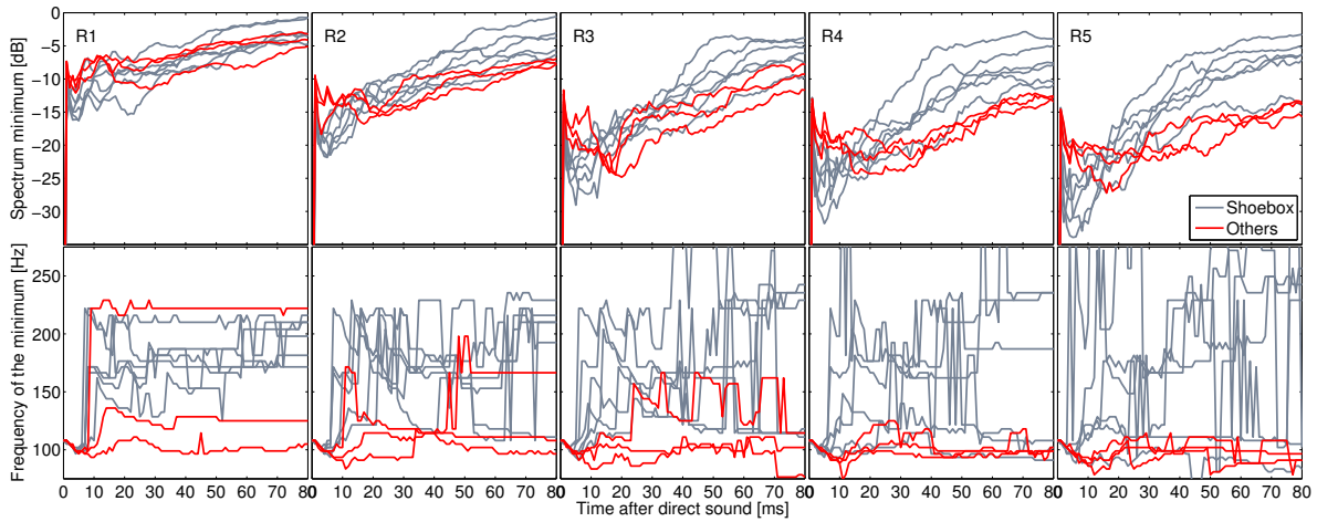
Figure 2 The spectrum minimum and its frequency at 1-ms time increments up to 80 ms after the direct sound in the shoebox vs. non-shoebbox halls at different receiver positions. The plot on the top shows the magnitude of the spectrum minimum and the bottom plot shows the frequency at which the minimum occurs. The frequency responses were 1/12-octave smoothed.
